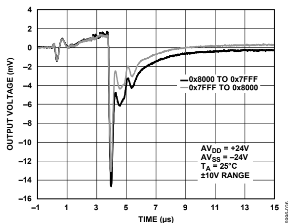
Figure 38. Digital-to-Analog Glitch
