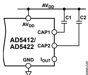
Figure 69. I_{OUT} Filtering Capacitors
