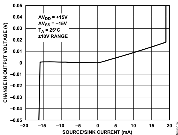
Figure 34. Source and Sink Capability of Output Amplifier, Full-Scale Code Loaded
