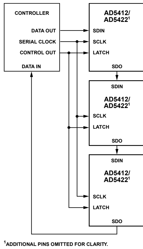
Figure 66. Daisy Chaining the AD5412/AD5422
